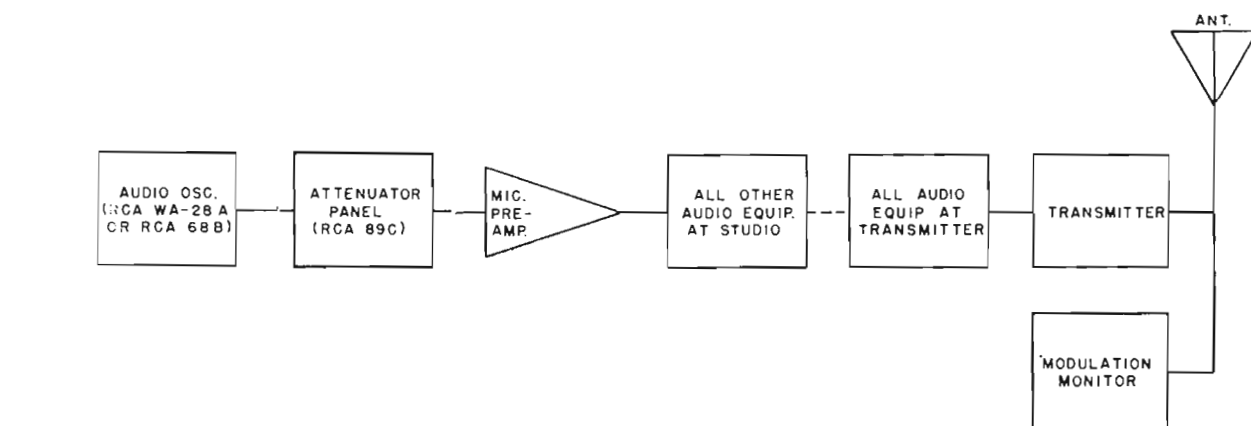
FIG. 2 (above). Block diagram of recommended equipment setup for measuring audio frequency response.
