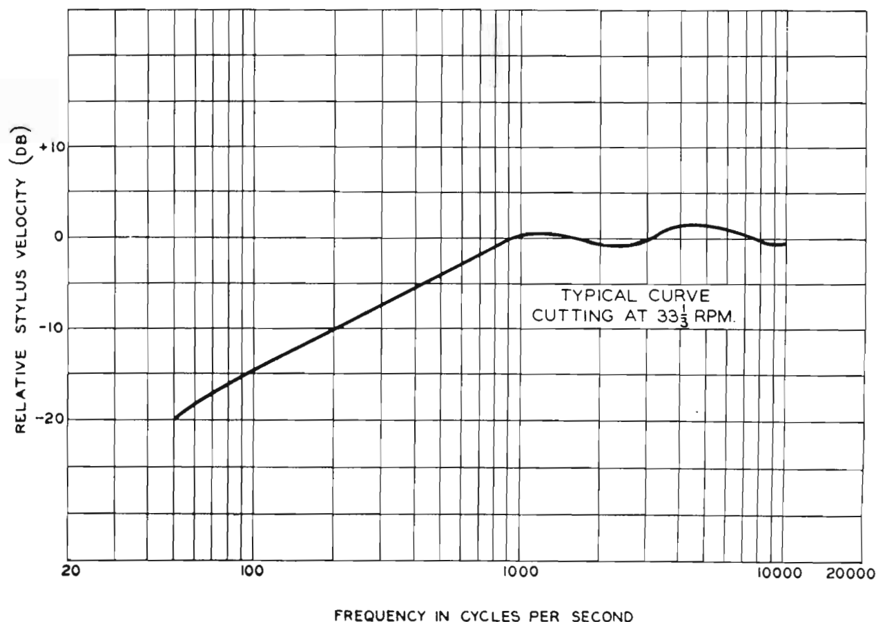
FIG. 7. (Below) Typical Response Characteristic While Cutting at an Average Diameter at 33 \frac{1}{3} r.p.m.
