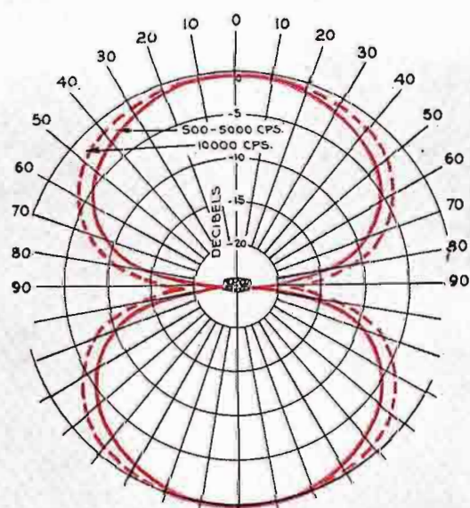
Directional characteristics of a typical KB-2C microphone.
