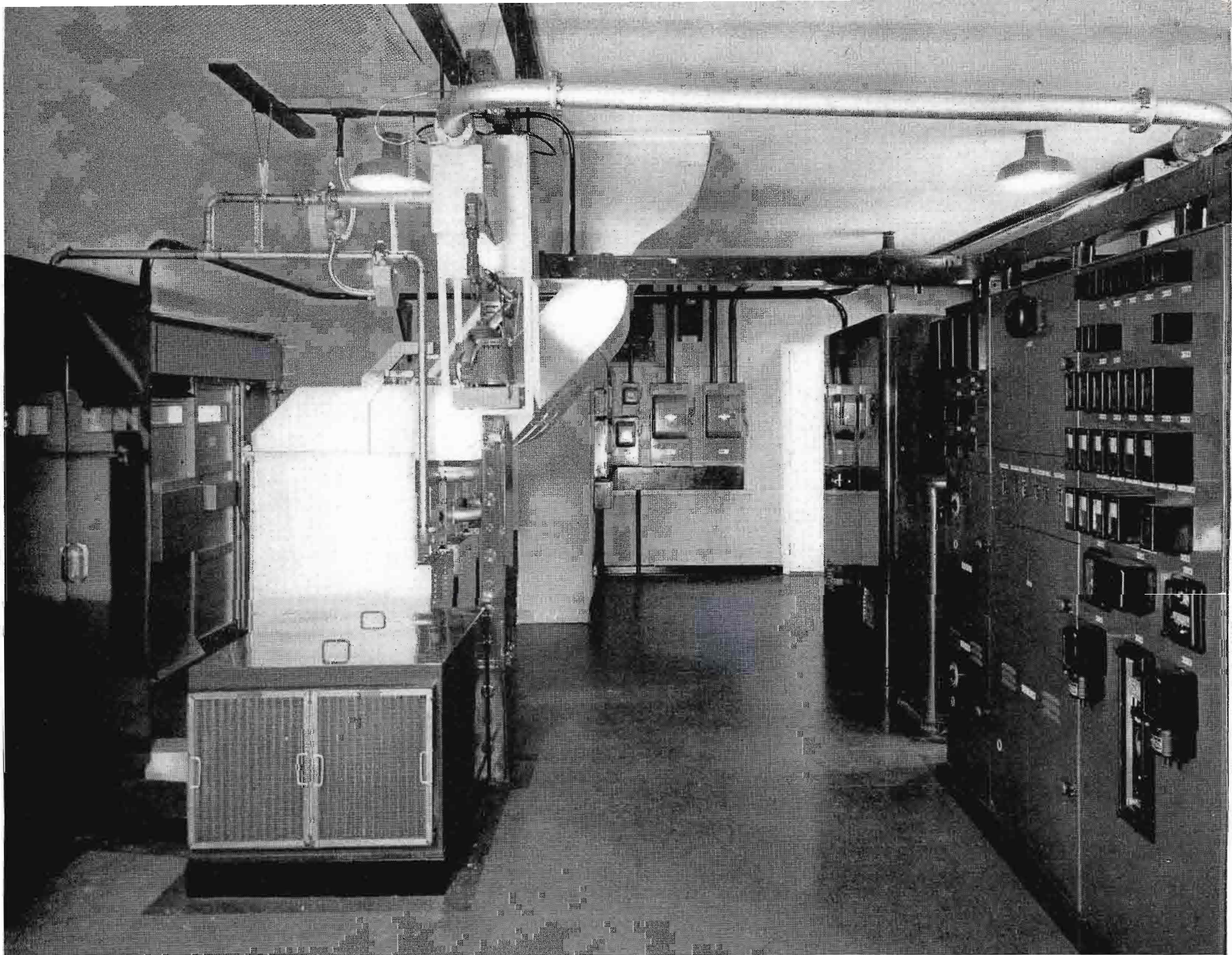
FIG. 5 (above). This view shows the entire BTF-50A, 50 KW FM enclosure. Low power r-f and exciter are at left, 50 KW grounded-grid amplifier at left center, and H-V rectifier and power and control units at the extreme right. Plenty of walk-around space is provided for every unit of the transmitter.
