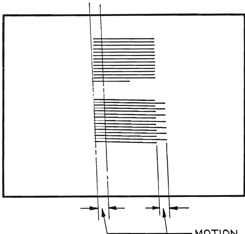
FIG. 3. Effect of horizontal motion of vertical edges in 2-to-1 interlaced system. Upper object stationary. Lower object moving to right.
