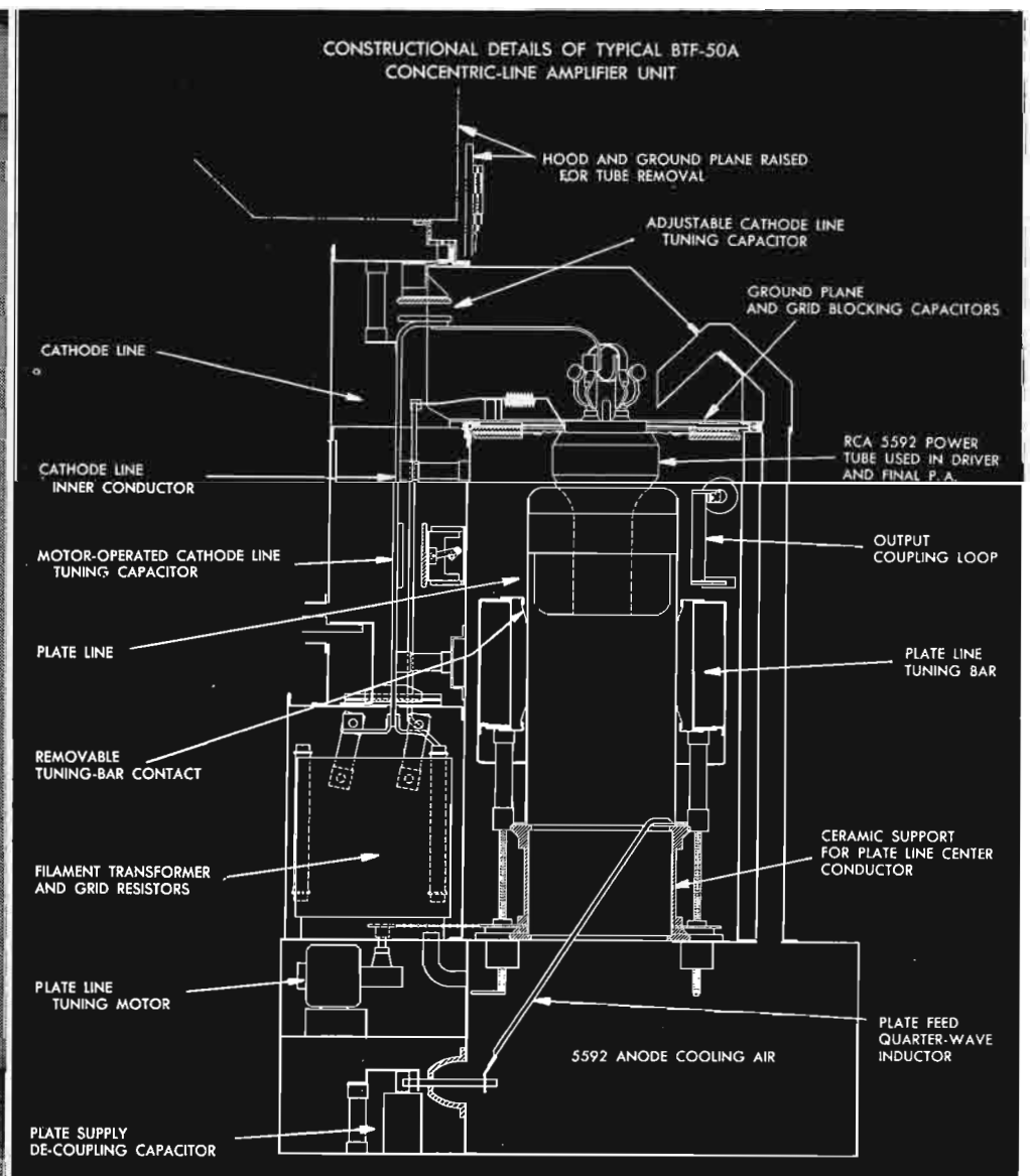
FIG. 9 (below). Mechanical sketch of a typical BTF-50A amplifier unit, illustrating details of construction and operation. All tuning is push button, motor-controlled from the transmitter front panel.
