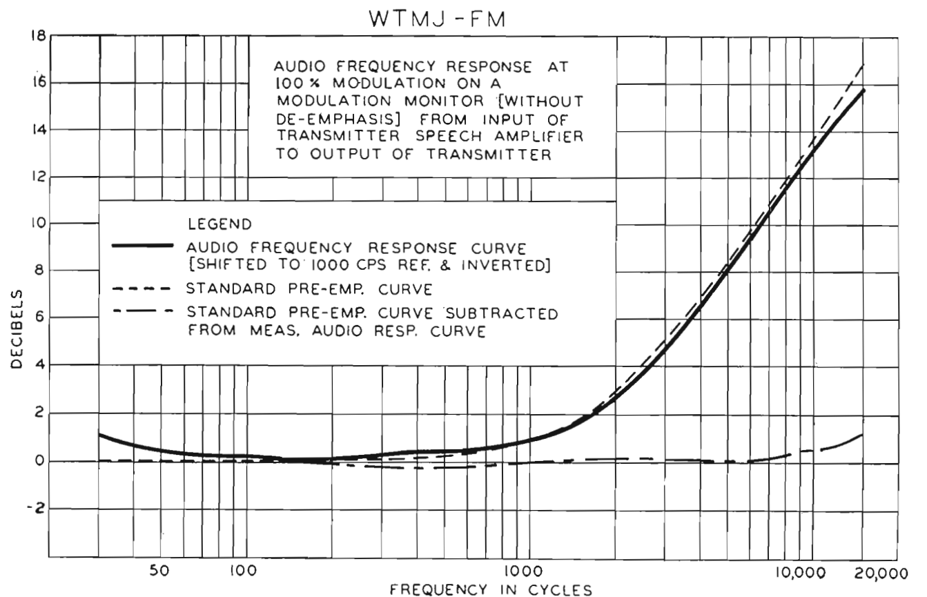
FIG. 12 (at right). Audio frequency response measurements taken on the WTMJ transmitter result in a curve which is essentially flat from 30 to 15,000 cycles.
