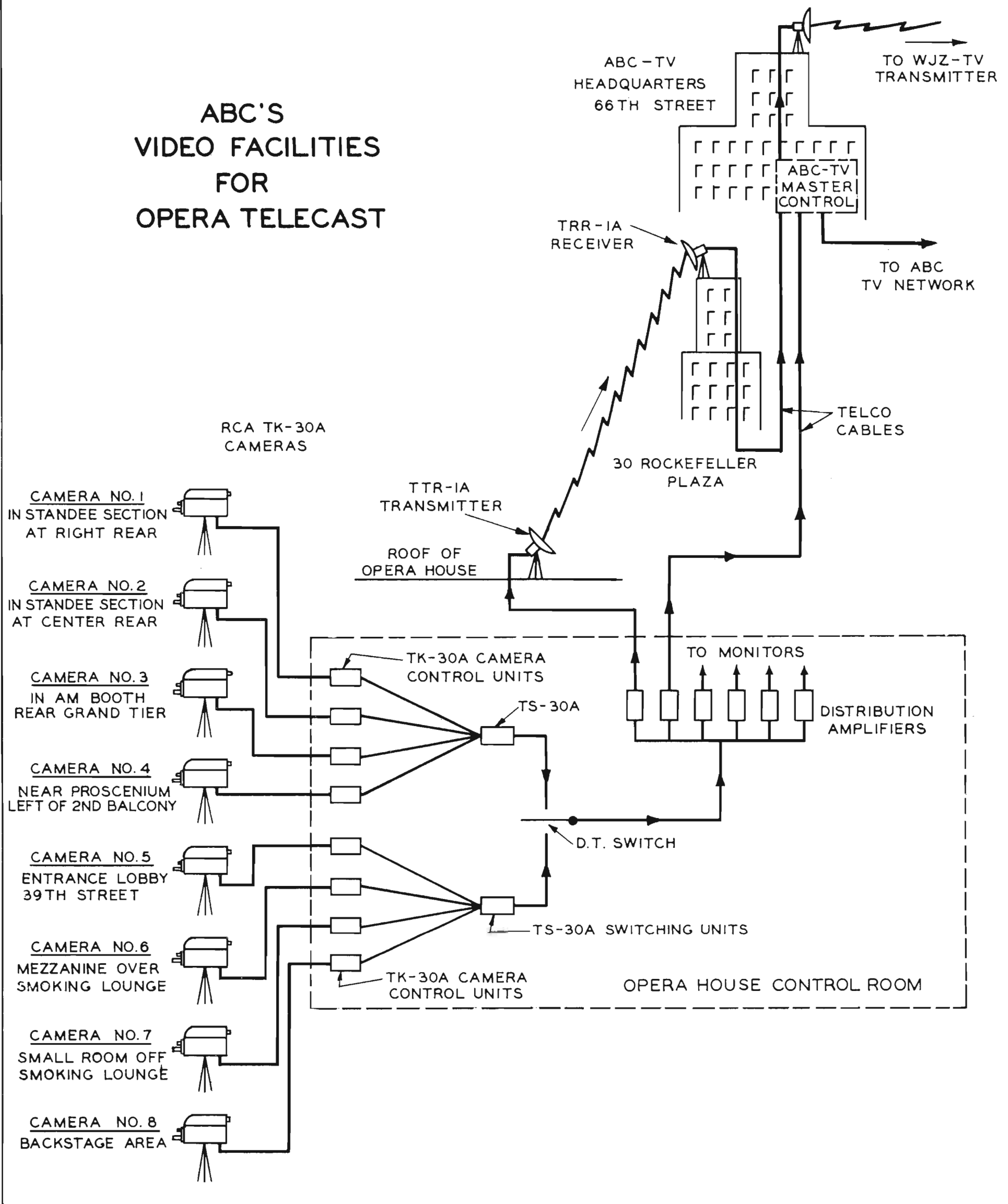
FIG. 6. Simplified schematic diagram of video facilities setup by ABC engineers for telecasting from the New York Metropolitan Opera House. Eight RCA cameras were connected by camera cables to eight camera control units located in the control room. Outputs of the camera controls were fed into two TS-30A switching units, as shown. The arrangement of cameras' mixing circuit was such that one group (Nos. 1, 2, 3 and 4) were in use during actual program, while the other group (Nos. 5, 6, 7 and 8) were in use before curtain time and during intermission. The output of either switching unit could be selected (by means of a double-throw switch) for transmission to the monitor system and transmitter lines. Two alternate methods of feed to the ABC TV headquarters at 66th Street were established in order to provide maximum insurance against program interruption.
