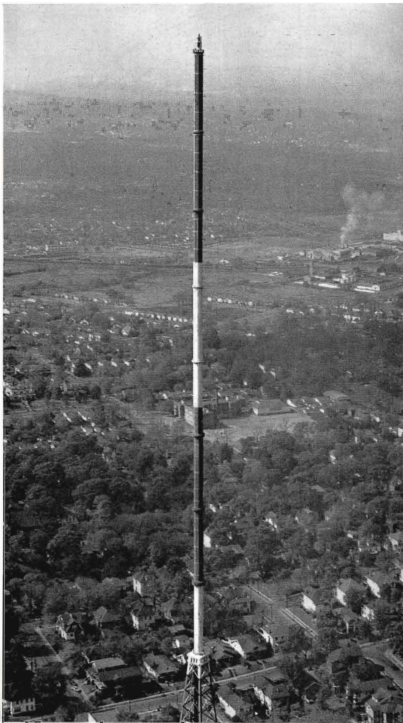
FIG. 3. Closeup of the high-gain, 8-section Pylon as installed on the 450 foot WBRC-FM tower.
