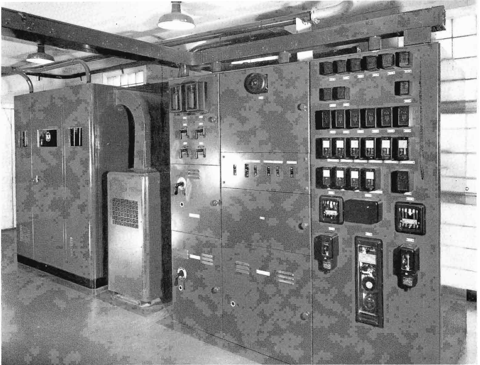
FIG. 16 (above). The complete high-voltage rectifier is housed in the cabinet at left above. At center is the H-V plate transformer; and at right, the transmitter power and control panels.
