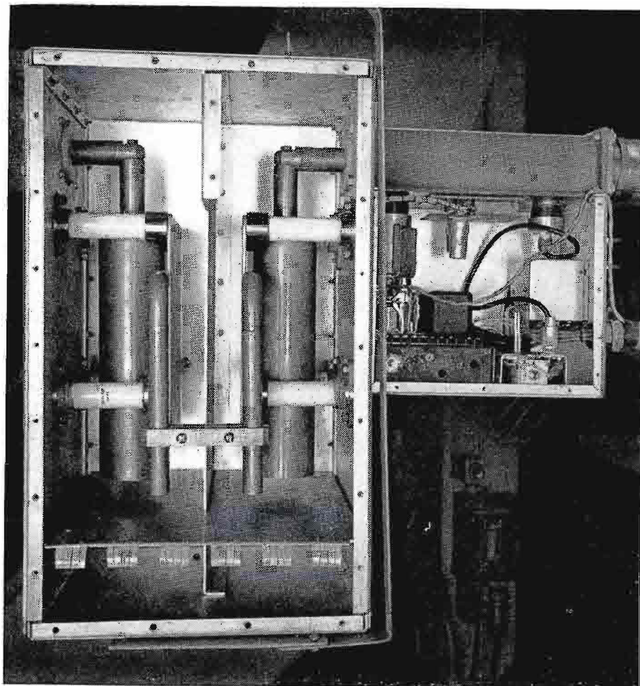
FIG. 13 (at right). Closeup view of the harmonic attenuator and transmission line monitor provided as a part of the transmitter equipment.
