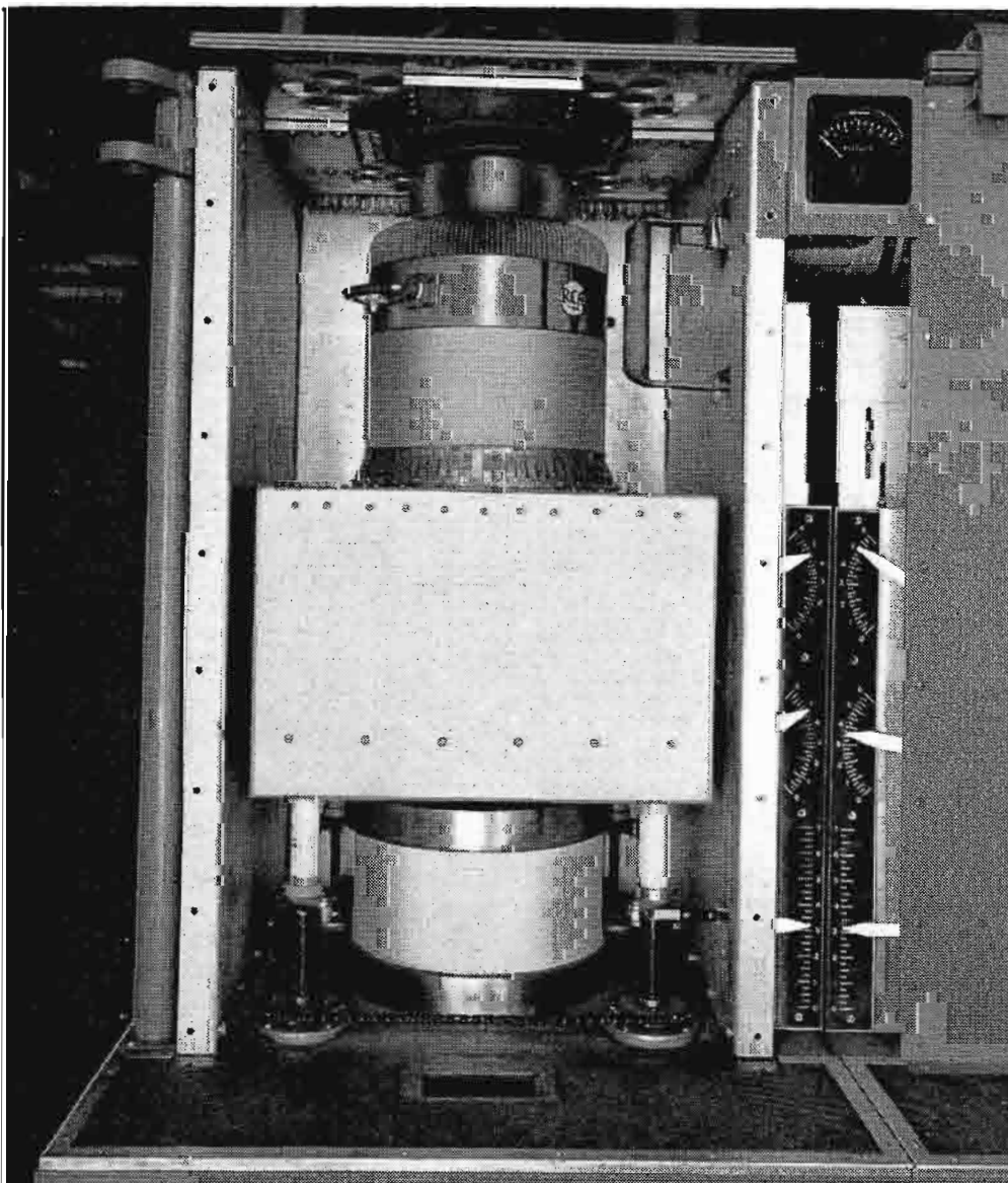
FIG. 8 (below). Closeup view of one section of the 50 KW P.A. unit with panel removed to show plate line, "shorting-bar," output coupling loop and balancing meter, as well as tuning indicators.
