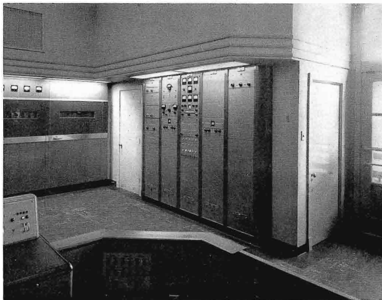
FIG. 5. The cabinet-type racks of audio input, monitoring, and test equipment are flush-mounted in a drop-wall as shown above. This type of construction gives the room a unified appearance and provides ample working room behind the equipment.
