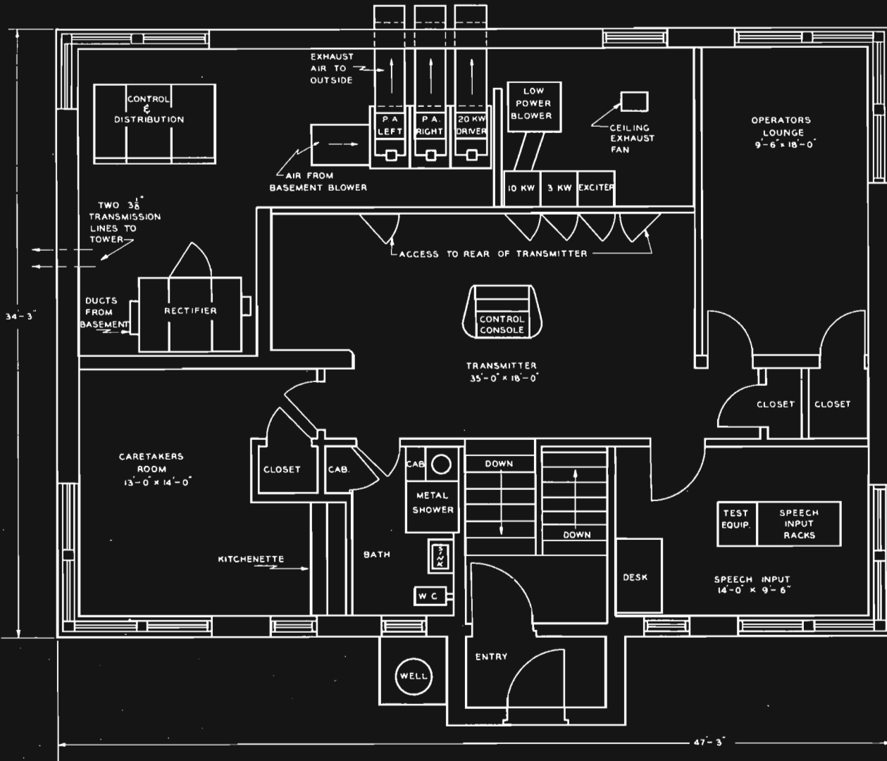
1 st FLOOR PLAN OF WTMJ-FM RICHFIELD, WISCONSIN TRANSMITTER BUILDING HOUSING RCA-BTF50A 50 KW FM TRANSMITTER
