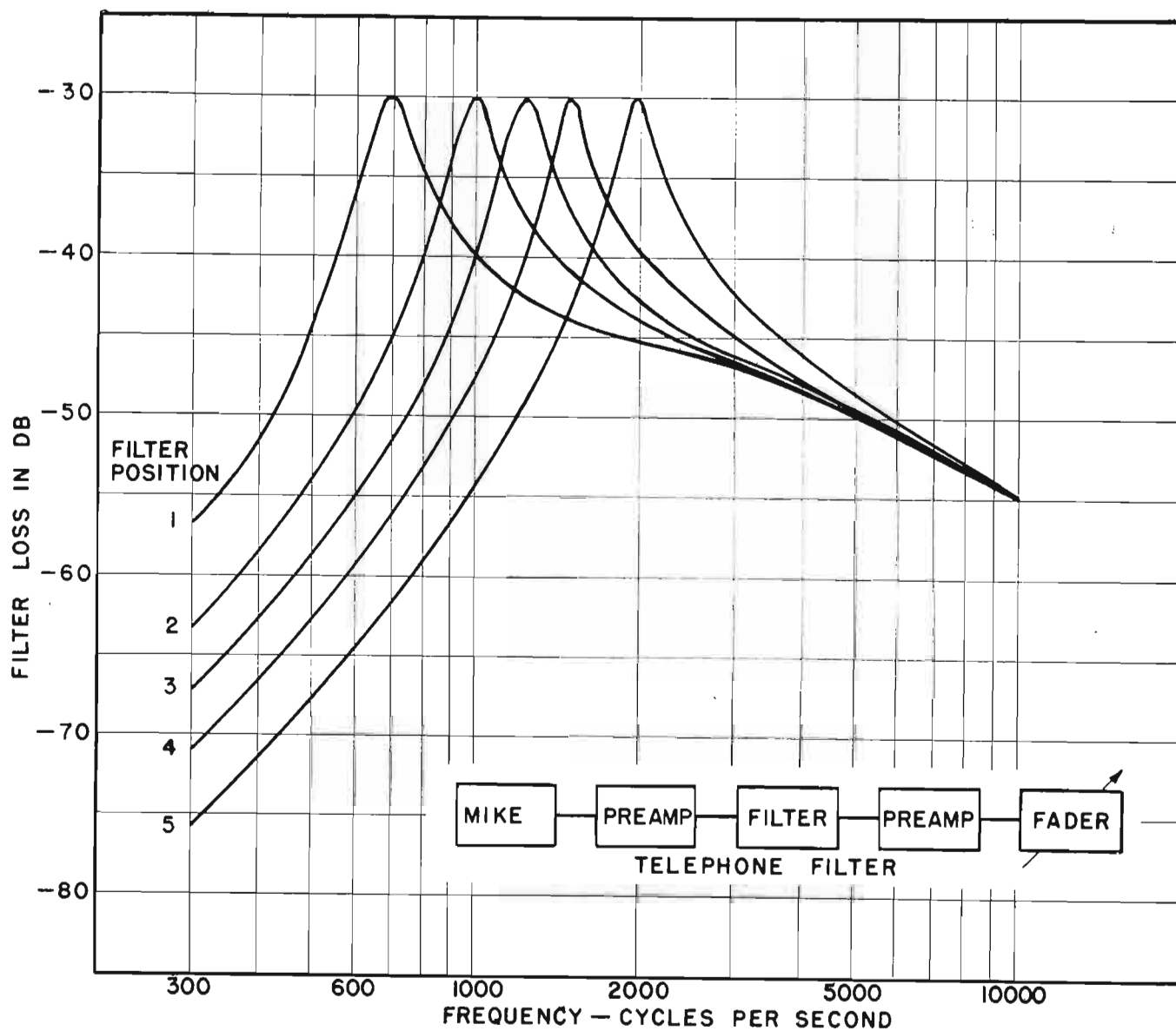
FIG. 6 (above). Typical telephone filter characteristics.
