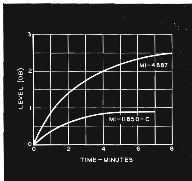
FIG. 6b. Continuous Application of 5000-Cycle Signal Causes a Greater Change in Level at 1000-Cycles. Note, However, the Improvement Obtained with the MI-11850-C over the MI-4887, which was not temperature controlled.
