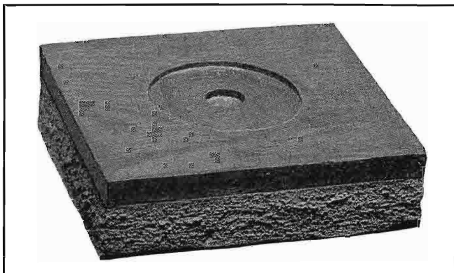
FIG. 4 (at left). Only three, easy-to-construct mounts like the one shown here are required. Note that top of shock mount is recessed to accommodate the turntable glide button and to avoid slippage of turntable.
