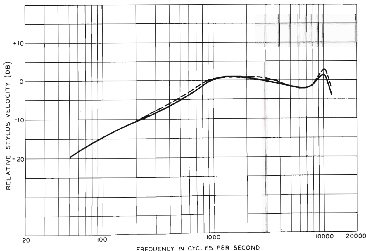
FIG. 5. (Below) Response Measurements Taken Six Months Apart—Note Only a Slight Change in Characteristic, an Improvement Resulting from Controlled Temperature Operation.
