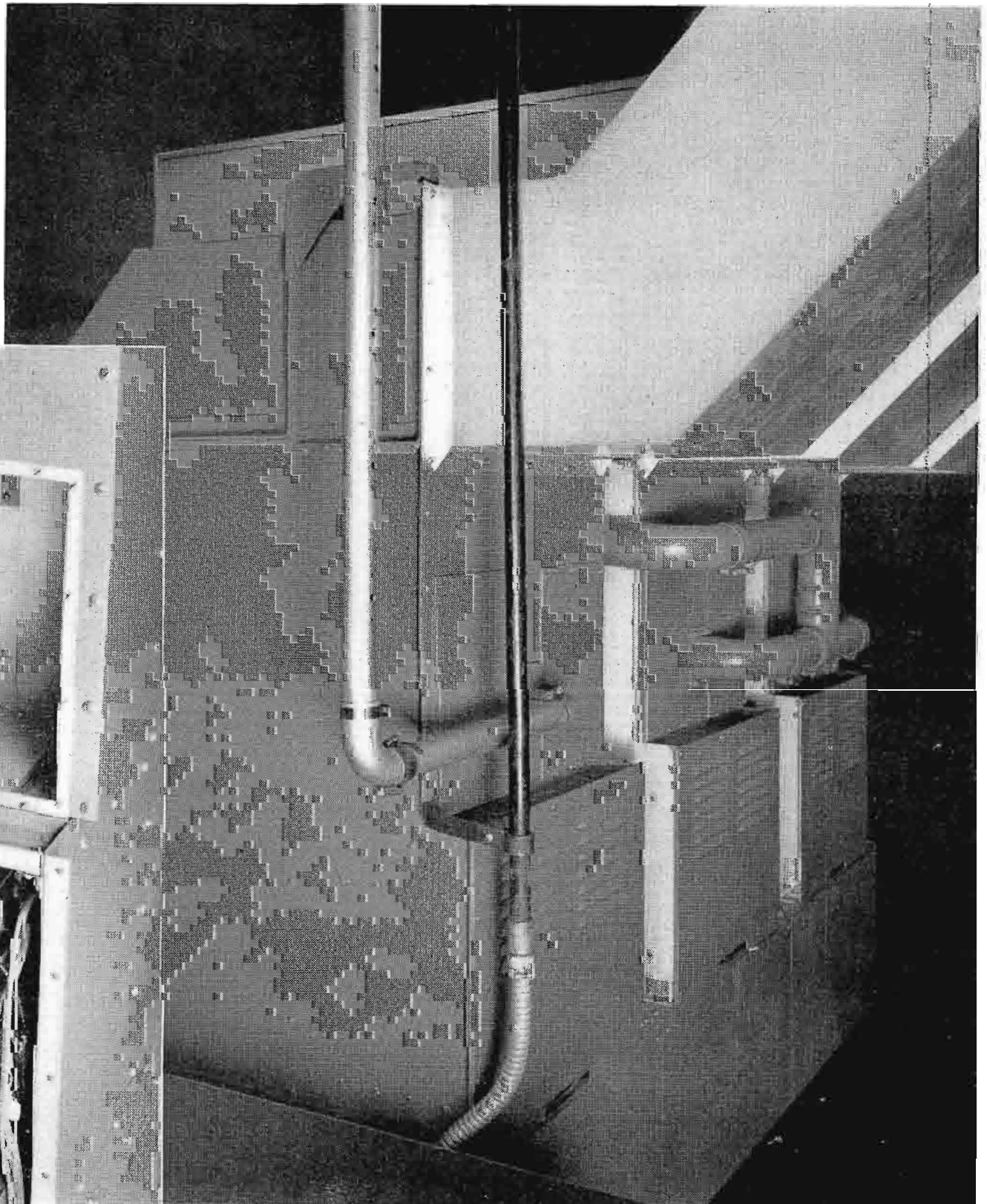
FIG. 10 (at right). Rear view of the 50 KW FM amplifier unit showing exhaust ductwork and coaxial lines.
