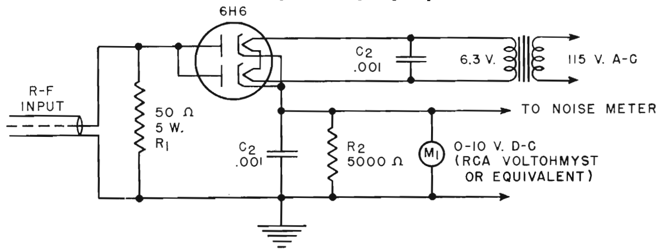
FIG. 3 (above). Schematic diagram of R-F rectifier which may be used for AM hum measurements.
