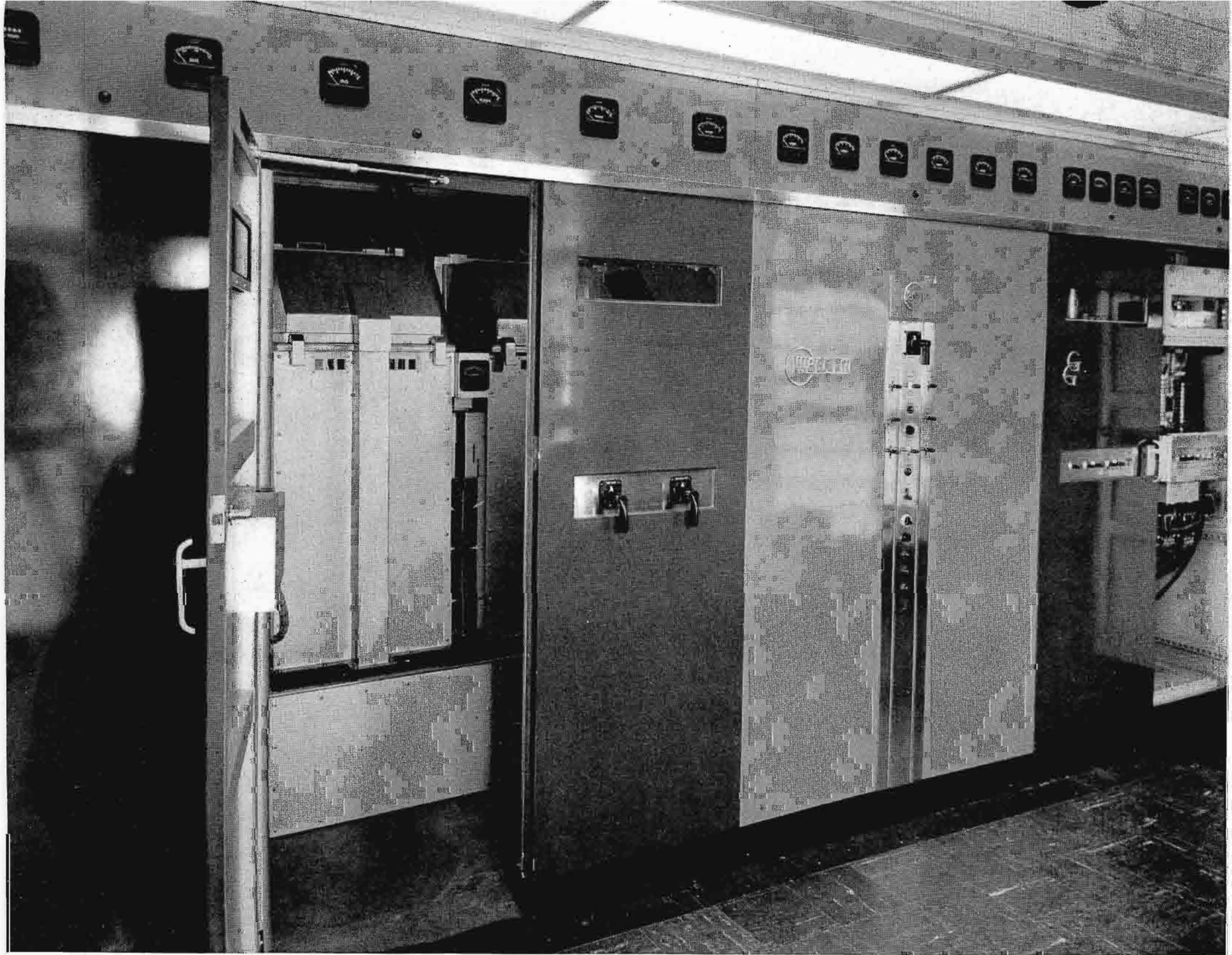
FIG. 3 (above). Front view of the WBRC-FM transmitter with doors opened to illustrate extreme accessibility. Note how 50 KW tanks at left are mounted so as to provide walk-around space.
