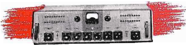
RCA Studio Consolette Type 76-C4. This flexible and easy-to-operate control unit performs all the audio amplifying, monitoring, and control functions of a TV station—large or small. Can be used for single- or two-studio operation, and for two transcription turntables.
