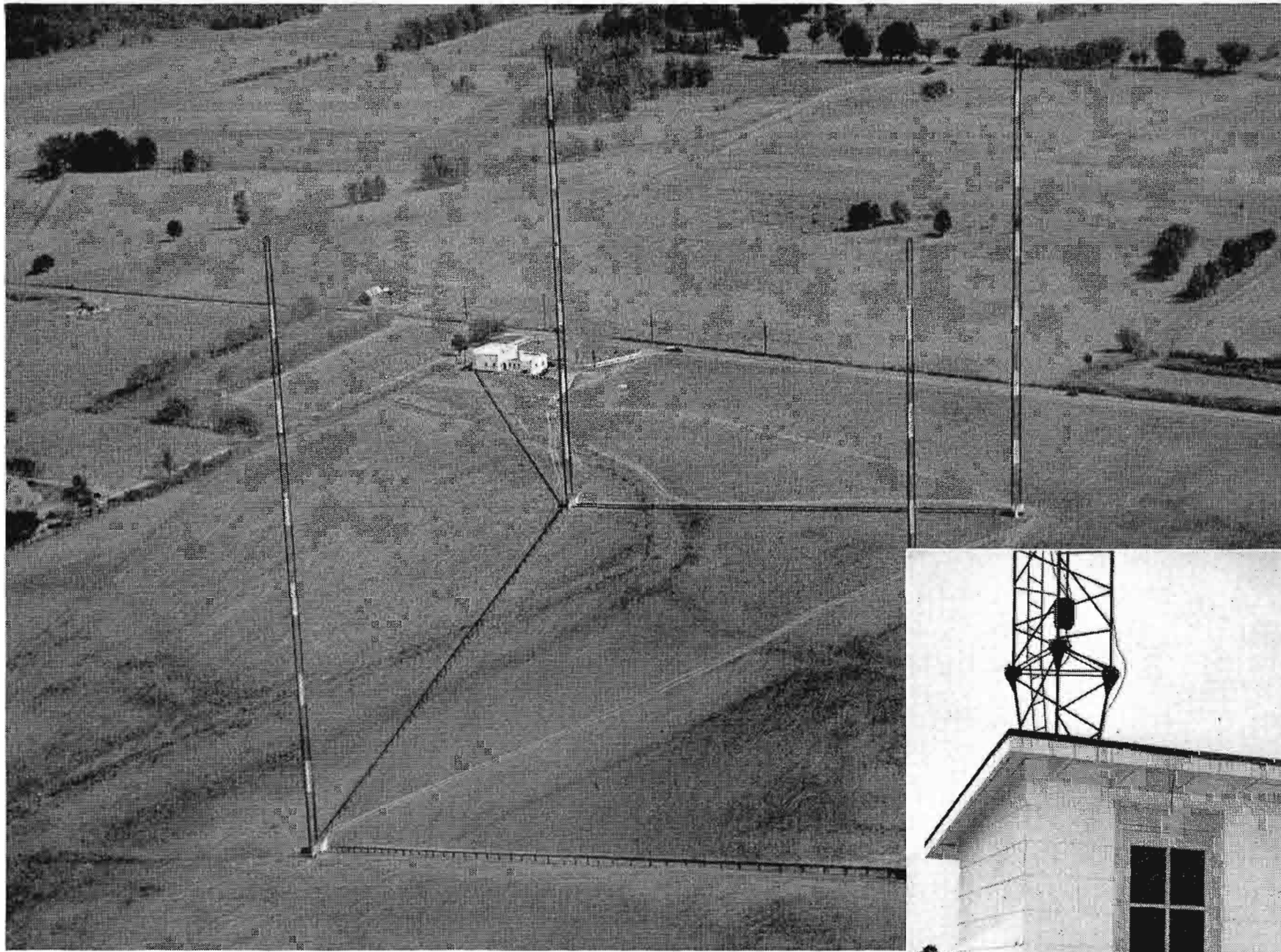
FIG. 6. Four guyed 400-foot towers arranged in a square make up the station's directive antenna array. Phasing equipment for the towers is housed alongside the 10 KW transmitter in a matched panel. The enclosure is standard RCA equipment which is added to transmitters when phasing equipment is employed. Inset shows one of the tower houses located at base of each antenna tower.
