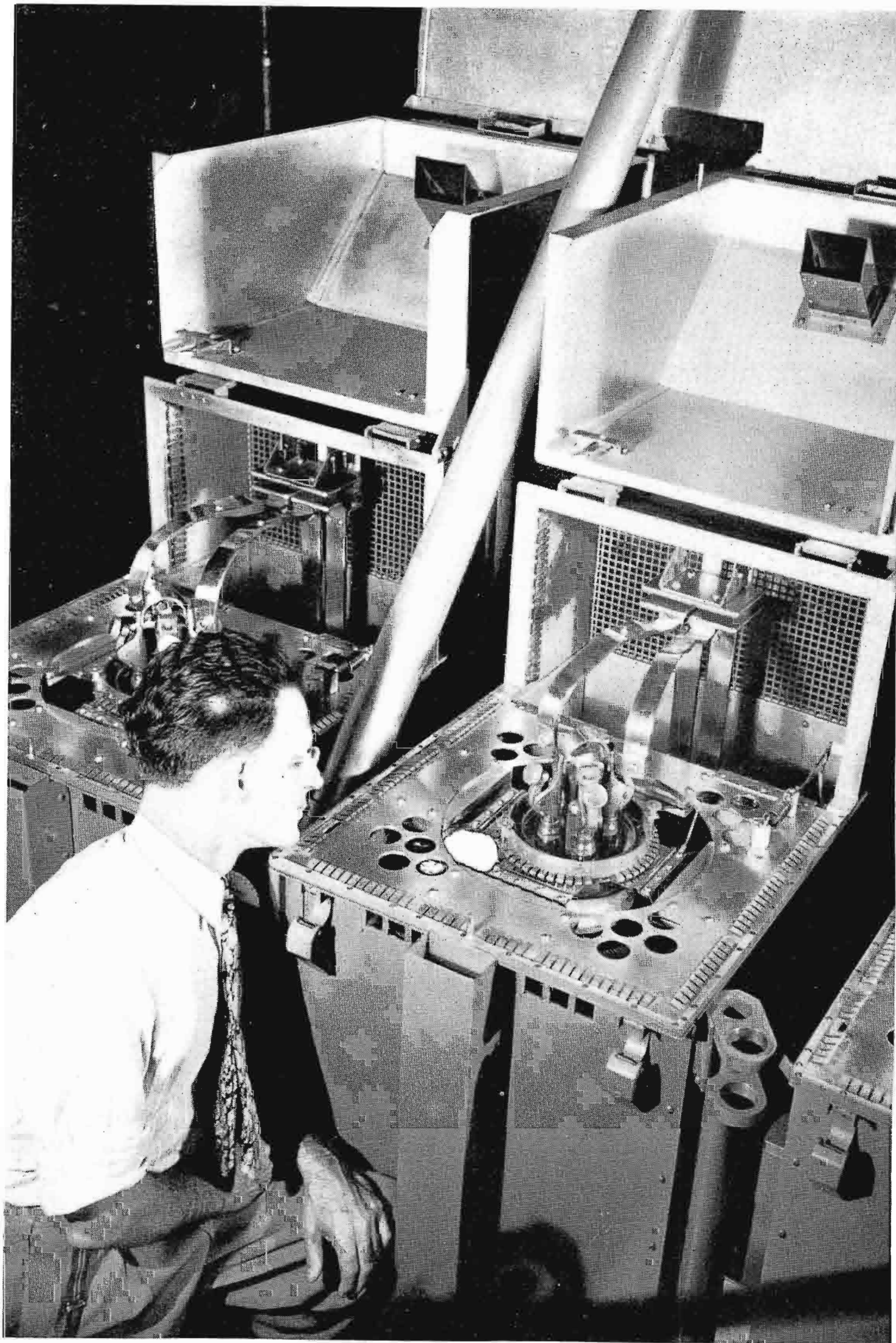
FIG. 6 (above). C. J. Starner inspecting one of the 50 KW FM tank units during engineering tests. The grounded-grid unit at left is the driver, and the two grounded-grid units (parallel-connected) at right form the final amplifier. Each concentric-line tank employs an RCA type 5592 tube. Each unit forms an integral part of the overall circuit. Complete shielding is provided. Neutralizing is not required.
