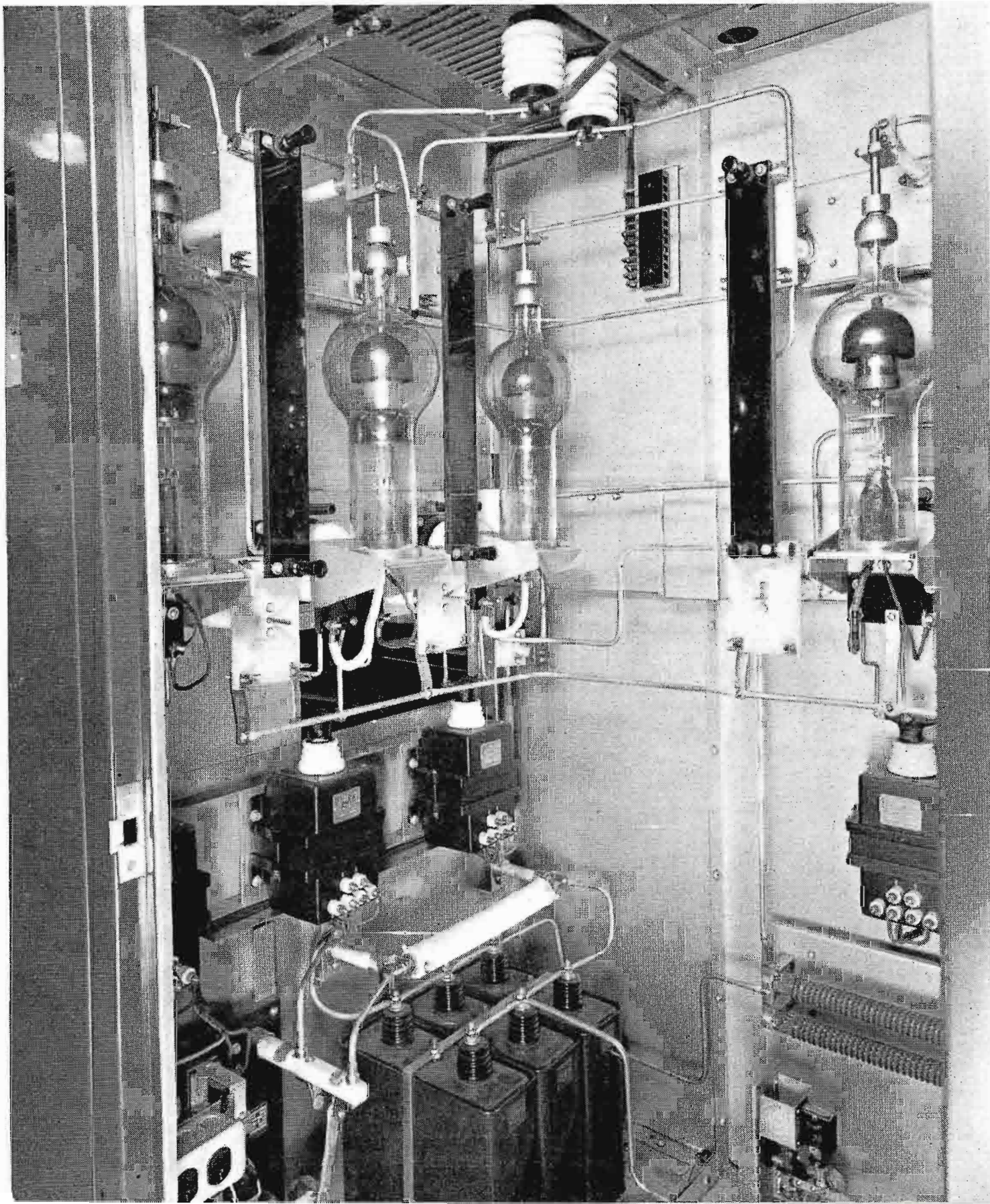
FIG. 15 (below). The high-voltage rectifier employs six long-life 857-B tubes and furnishes plate voltage for entire transmitter. A pre-heated spare which may be switched in place of any one of the operating tubes is provided. Full width door provides walk-in access to all rectifier components.
