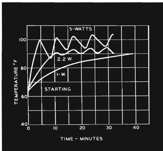
FIG. 4a. (Above) Warm-Up Time and Temperature Fluctuations at Damper Block for Different Heater Dissipation.
