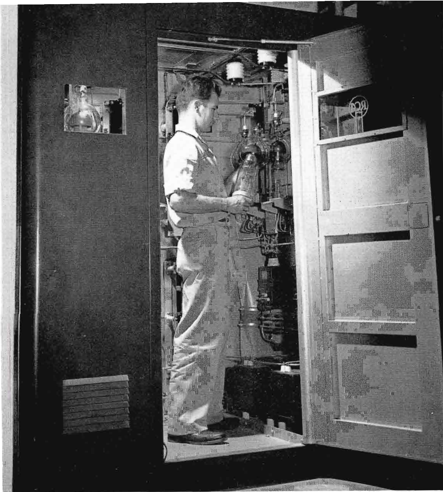
FIG. 9 (at left). WTMJ-FM engineer, Raymond Hernday, is shown installing an 857-B rectifier tube. This photo shows the "walk-in" type construction used for ease of operation and maintenance of all components of the 120 KVA rectifier unit. This rectifier supplies plate voltage to all power amplifier tubes down to and including the \frac{1}{4} KW amplifier.
