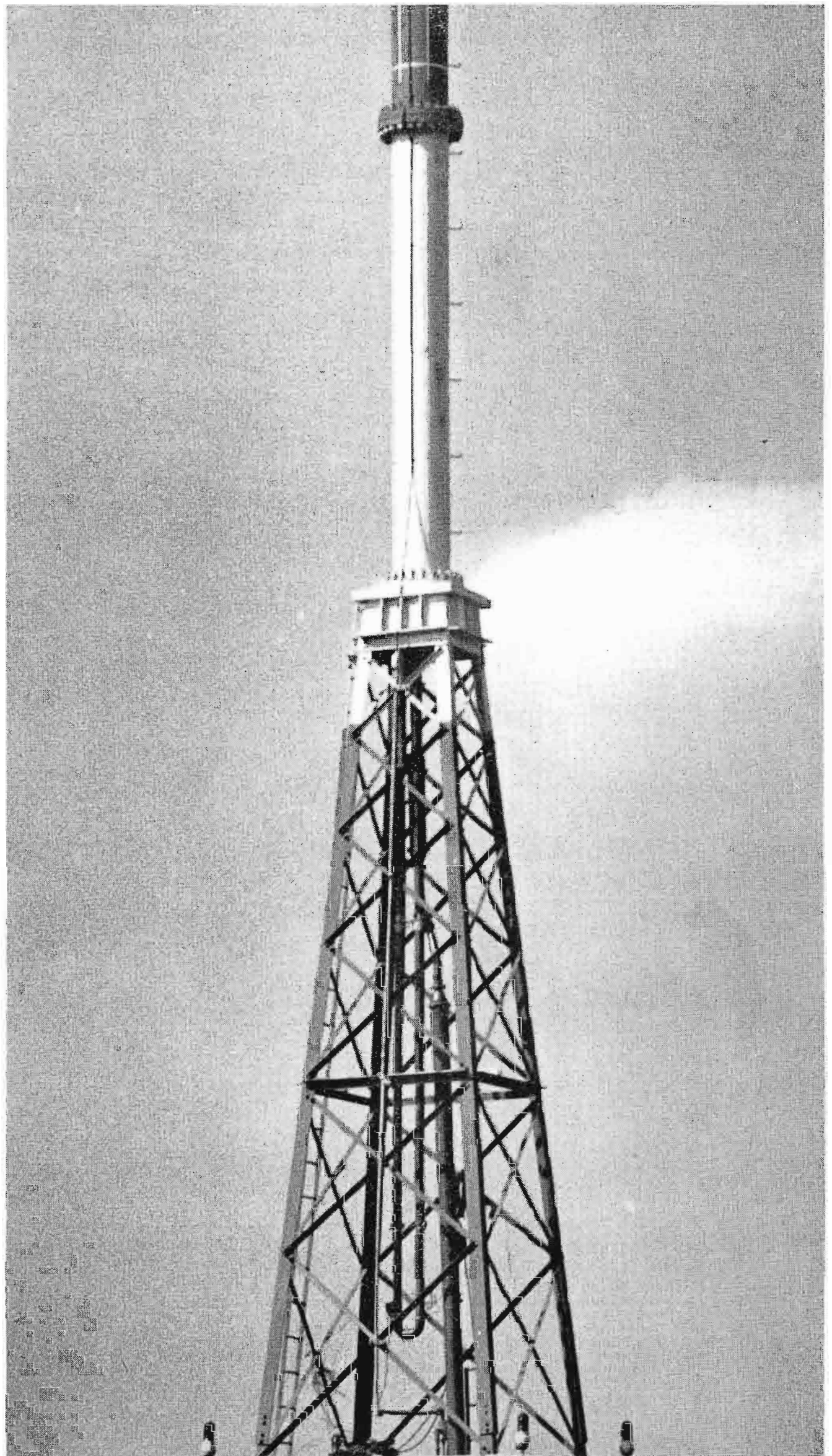
FIG. 4. Phasing and matching units are installed at the tower top as shown in this closeup view. Trombone phasing adjustment used for optimum vertical pattern tilt is visible within the tower.
