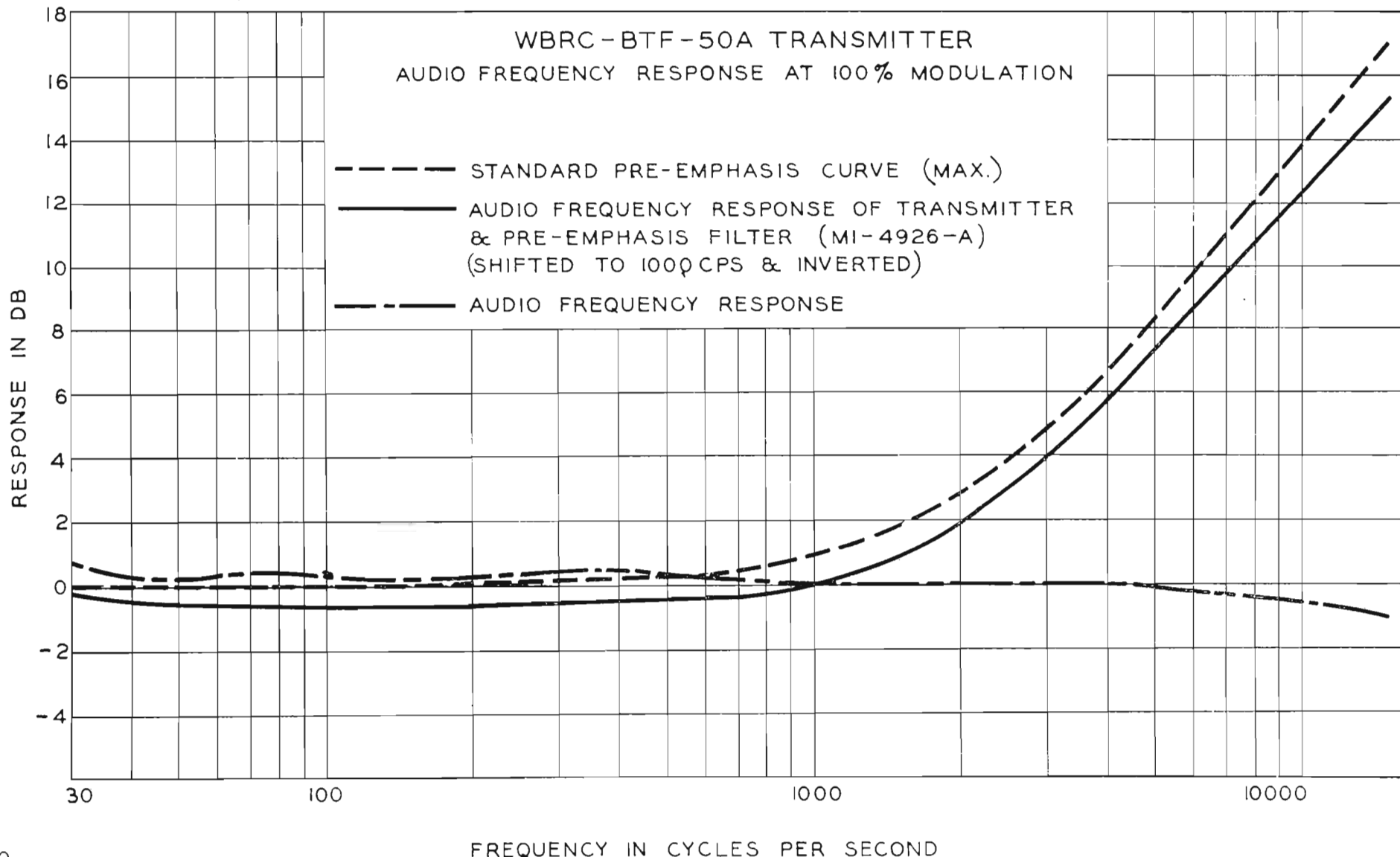
FIG. 7 (below). Frequency response curves taken on WBRC-FM's 50 KW transmitter show response to be essentially flat from 30 to 15,000 cycles. (Measurements were taken with antenna load, and isolation or r-f filtering were not necessary.)
