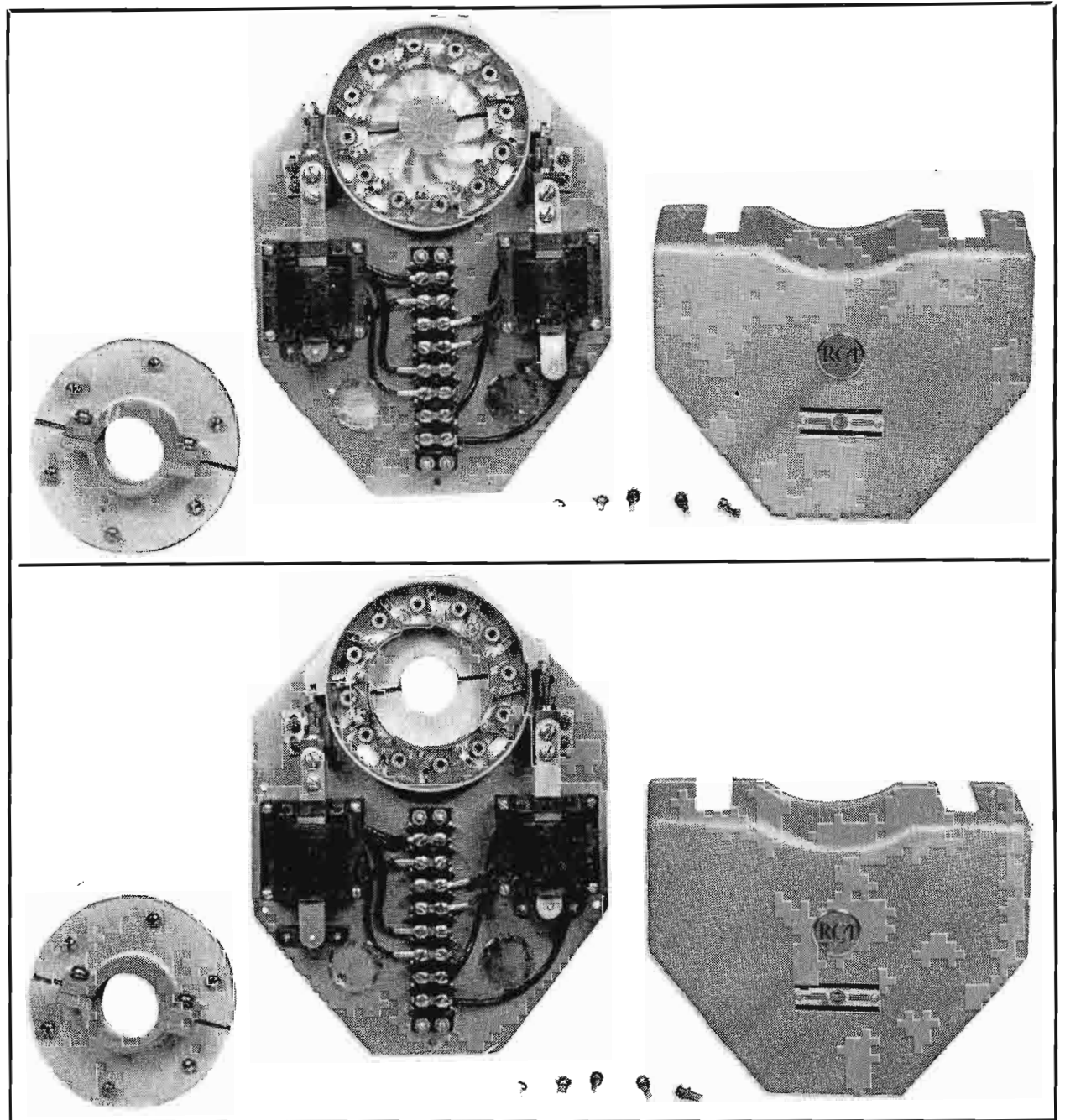
FIG. 3 (above). View of the shorting switch in the "open" position. Mounting flange is shown at left and protective cover at right.
