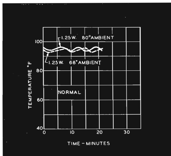
FIG. 4b. Temperature Fluctuations after Suitable Warm-Up Time.
