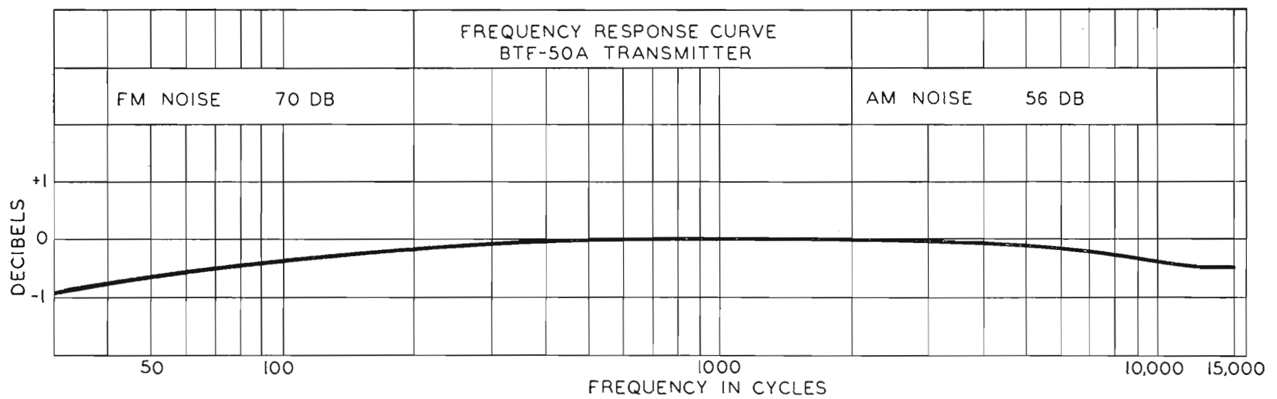
FIGS. 17 and 18 (below). Frequency Response and Audio Distortion curves plotted from engineering test floor data. Response is flat within \pm 1 db from 30 to 15,000 cycles and distortion less than 0.75%.
