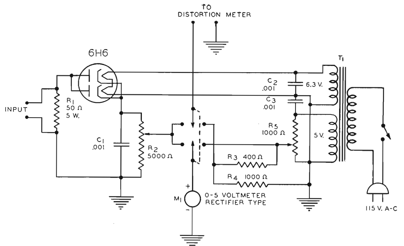
FIG. 14 (above). Schematic diagram for a diode rectifier for measuring AM hum and noise. Note that this equipment will give direct readings when used with any noise meter.
