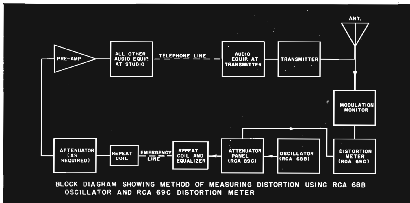
FIG. 1b (left). Equipment setup for measuring distortion, when transmitter is located adjacent to studio, or where a second line with low noise and distortion is available.
