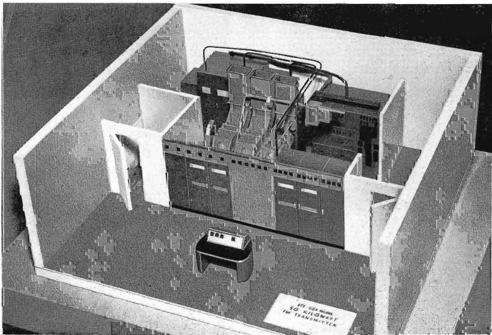
FIG. 3 (at right). This model of the 50 KW FM transmitter made during early design stages shows how the entire BTF-50A equipment may be installed on one floor. Entrance doors (at left) to the H.P. blower room and (at right) to the overall transmitter enclosure provide complete walk-in accessibility.
