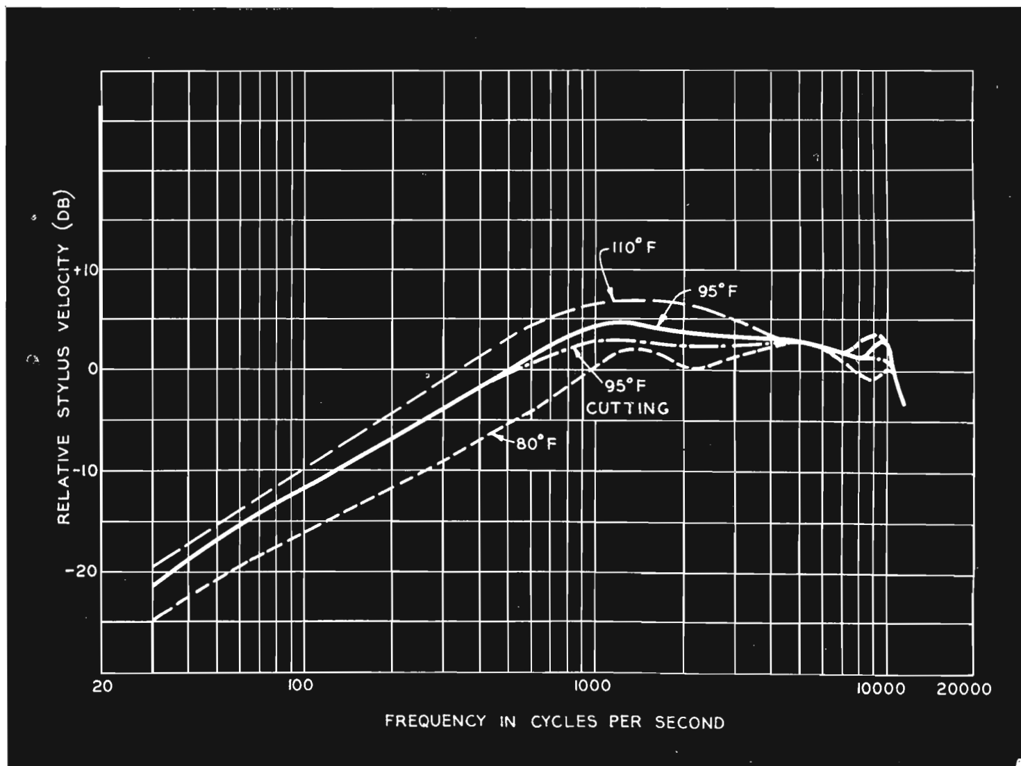
FIG. 3. (Below) Change in Response with Temperature.
