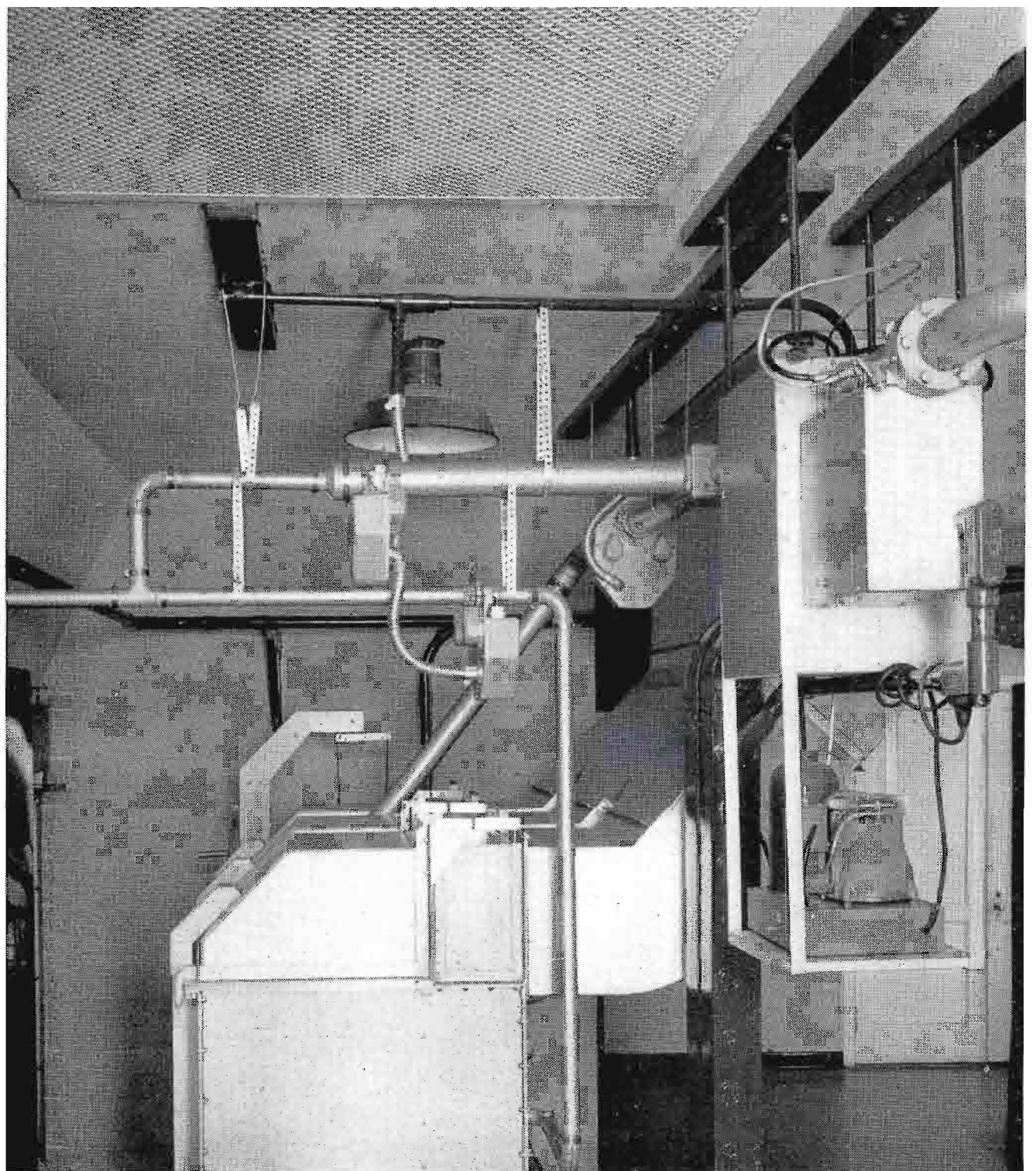
FIG. 8 (above). Closeup of a portion of the 50 KW FM amplifier unit showing the transmission-line power cutback switch arrangement. (Visible in center of photo.) The transmission line monitor and harmonic filter are shown at extreme right.
