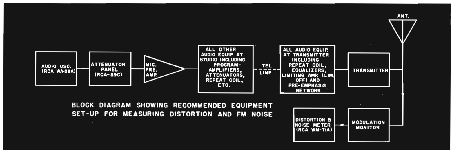
FIG. 1a (right). Arrangement of test equipment which may be used for distortion and FM noise measurements, when transmitter is located remote from studio.
