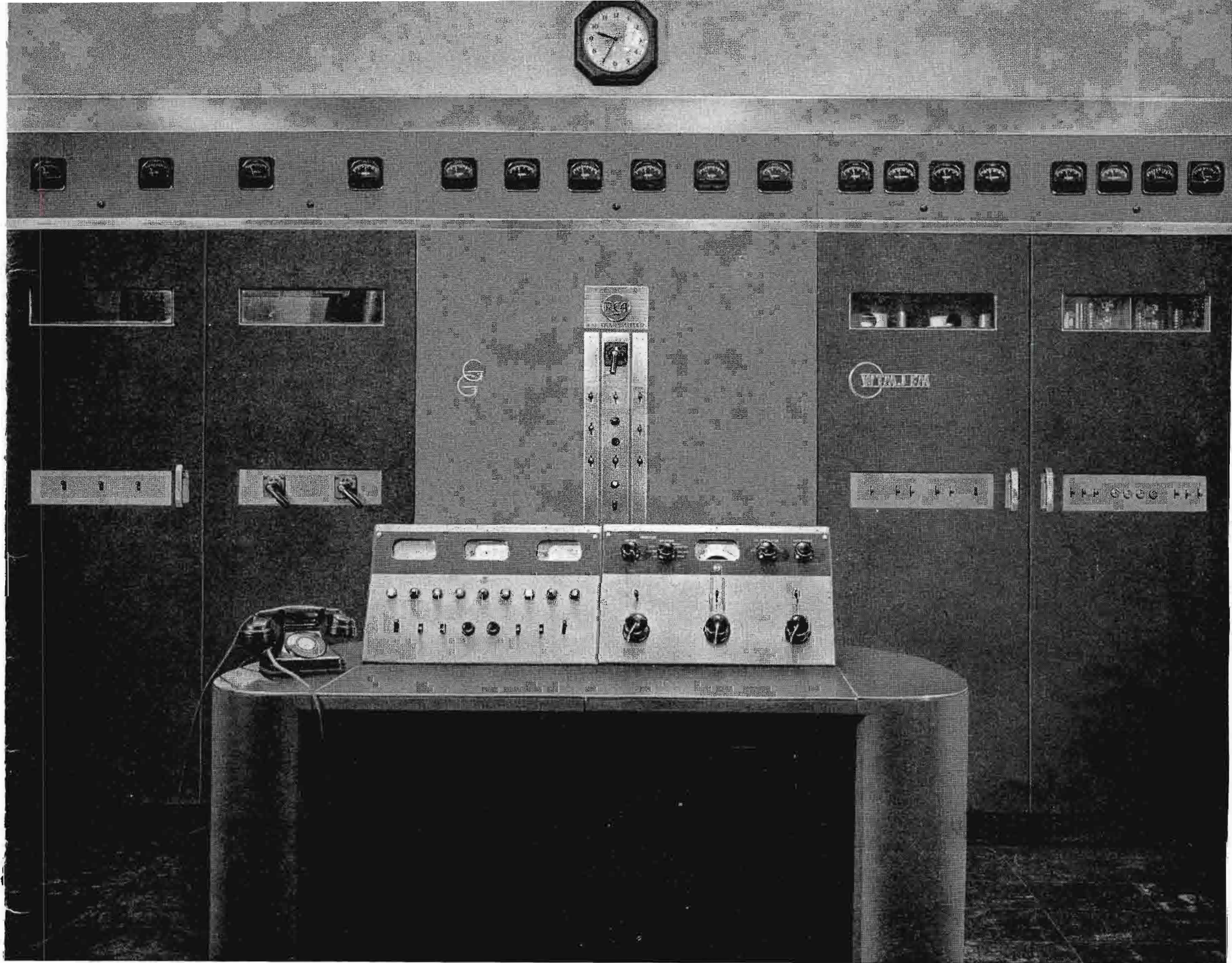
FIG. 2 (above). The final, commercial design 50 kilowatt FM transmitter as installed at WTMJ-FM, Milwaukee. The unified-front panel is finished in a two-tone umber gray to match companion equipment. In foreground is the BTC-1A supervisory console supplied with the transmitter.
