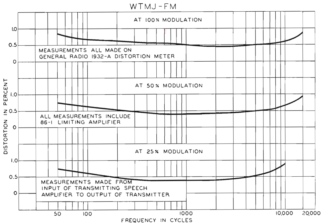
FIG. 11 (at left). As the distortion curves at left illustrate, overall performance of the WTMJ transmitter is well within the FCC distortion limit of 1½% from 30 to 15,000 cycles.
