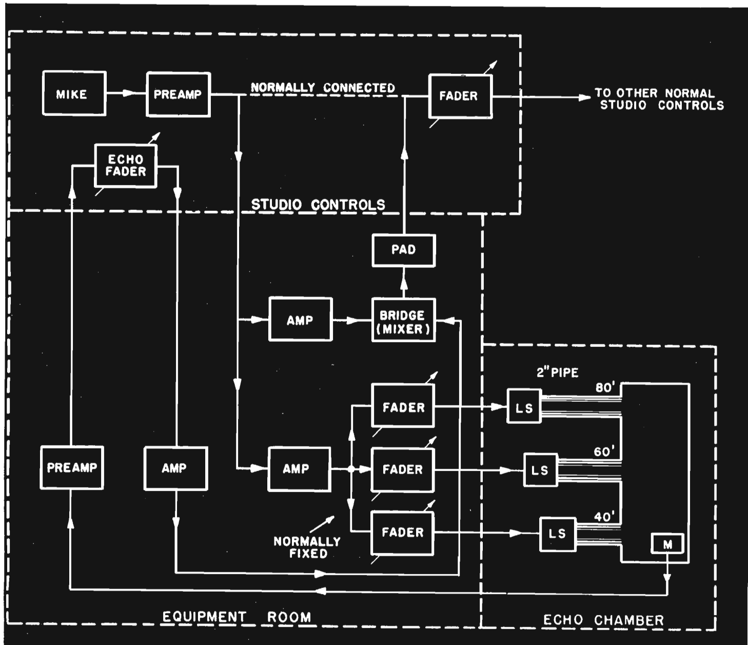
FIG. 7 (below). Echo chamber line-up.
