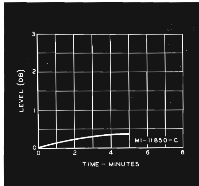
FIG. 6a. (Above) Continuous Application of Sine-Wave Signal Causes Some Increase in Recording Level at 1000-Cycles.
