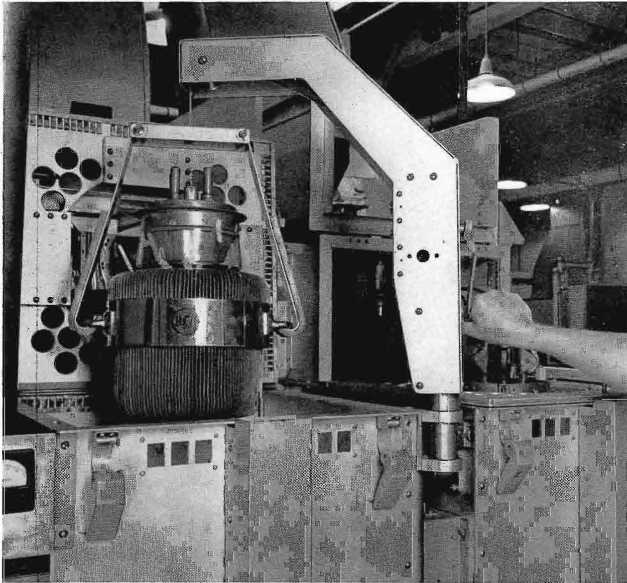
FIG. 8 (below). Closeup view of one section of the 50 KW P.A. unit with panel removed to show plate line, "shorting-bar," output coupling loop and balancing meter, as well as tuning indicators.
