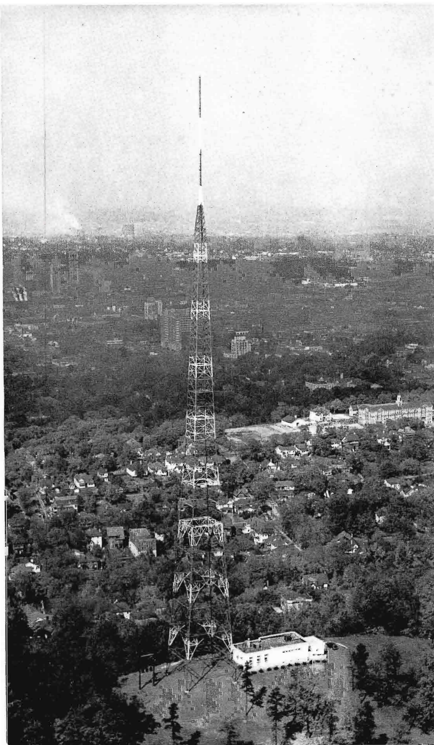
FIG. 1. Aerial view of WBRC-FM 8-section Pylon antenna installation, showing Birmingham in the background and the WBRC-FM transmitter house at the tower base.
