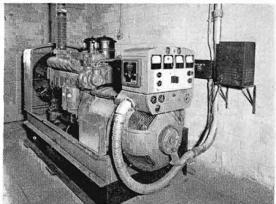
FIG. 8. To insure uninterrupted broadcast service, WMPS installed this 60 KW Diesel auxiliary generator for use in case power fails.
