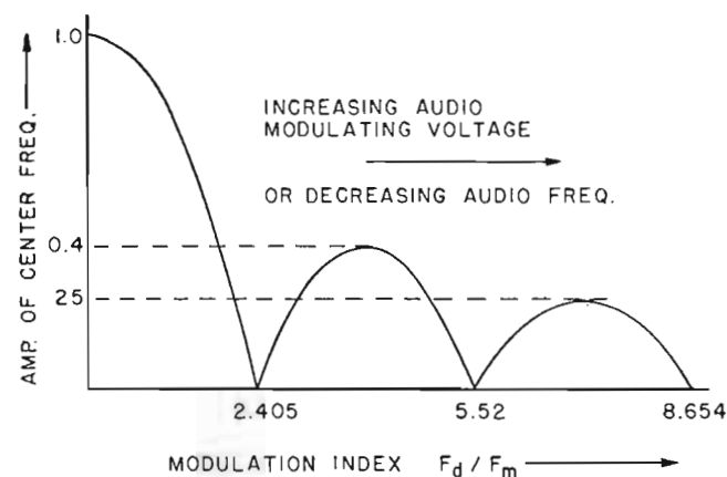
FIG. 11 (above). Center-frequency wave amplitude variation with increasing audio modulating voltage.
