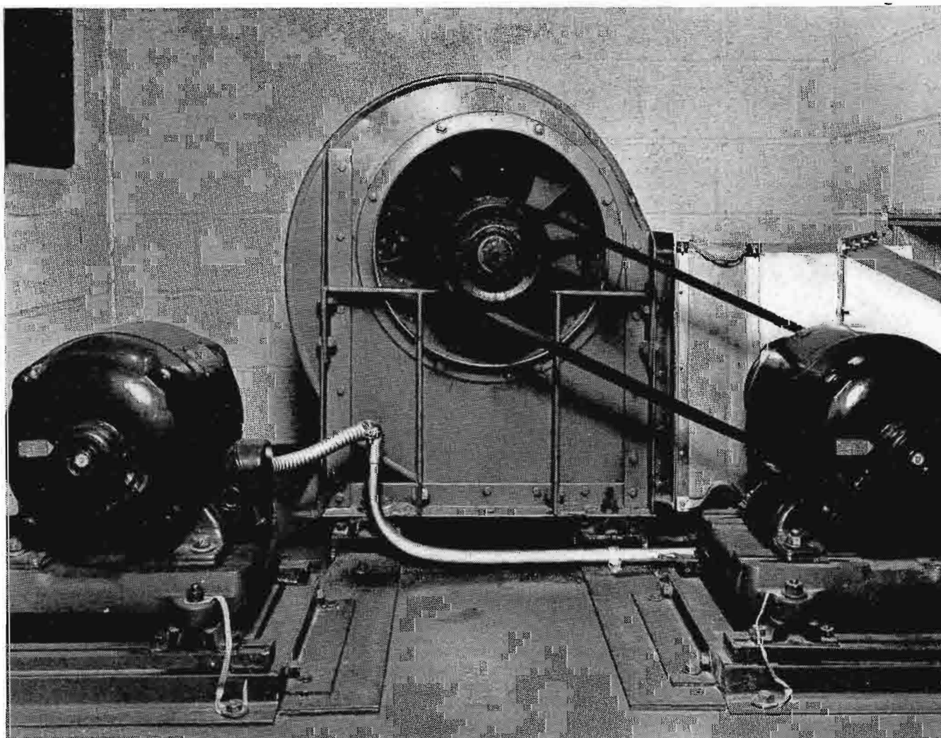
FIG. 12 (below). View of the blower and motors used for supplying cooling air to the 50 KW driver and final amplifier unit.
