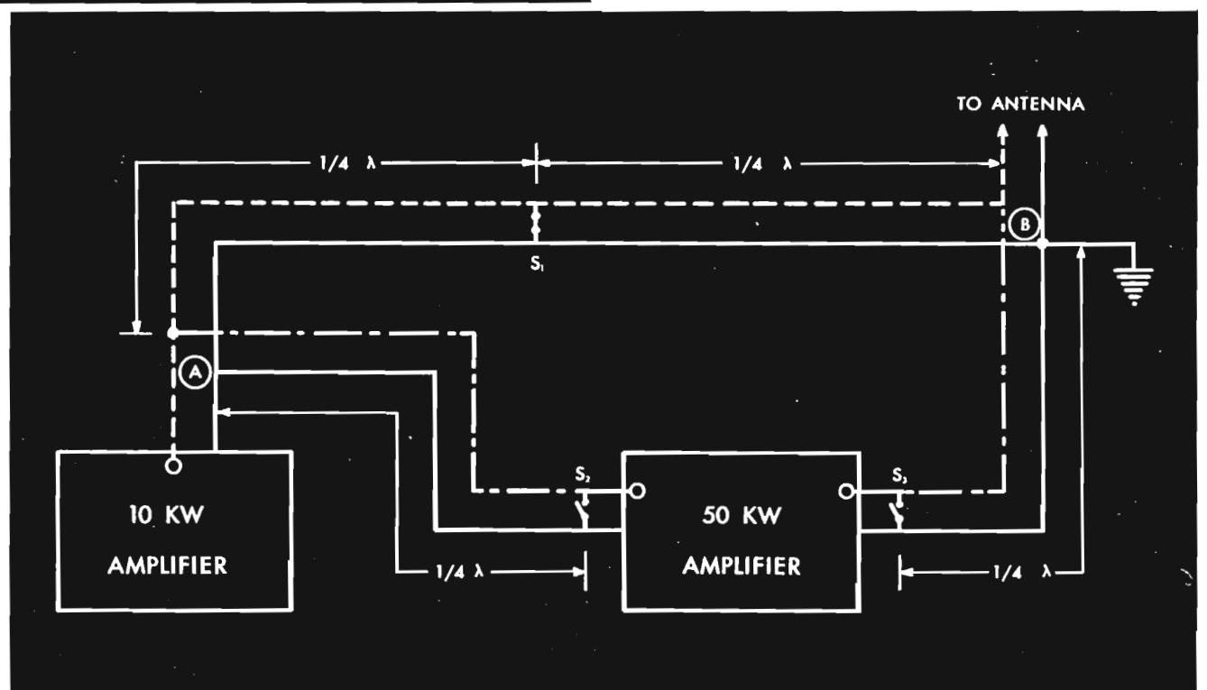
FIG. 5 (at right). High-Power Operation . . . During regular operation (at full power output) switch S_1 is closed and switches S_2 and S_3 are open. S_1 shorts the direct line between the 10 KW amplifier and the antenna (dotted) and causes the output of the 10 KW amplifier to be fed to the input of the 50 KW amplifier. The output of the 50 KW amplifier feeds the antenna through the line indicated (in long dashes). S_1 , being a quarter wave from point A and B, reflects infinite impedance at these points and hence does not affect normal operation.
