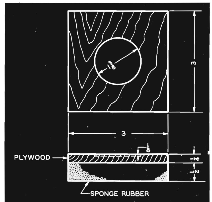
FIG. 3. Sketch showing constructional details of the sponge-rubber shock mountings, which are made of inexpensive, easily-obtained materials.
