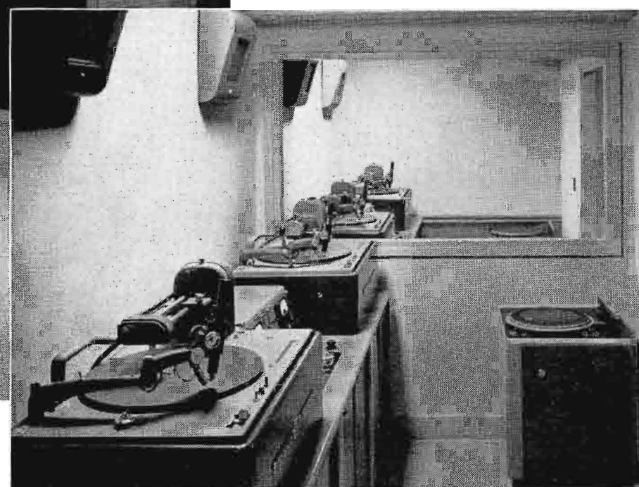
FIG. 4. An interesting mural consisting of a montage of radio equipment decorates the corridor leading to the recording rooms. The inset shows four RCA 73-B Professional Recorders and 70-D Transcription Turntables which are used by CMQ in its deluxe installation.
