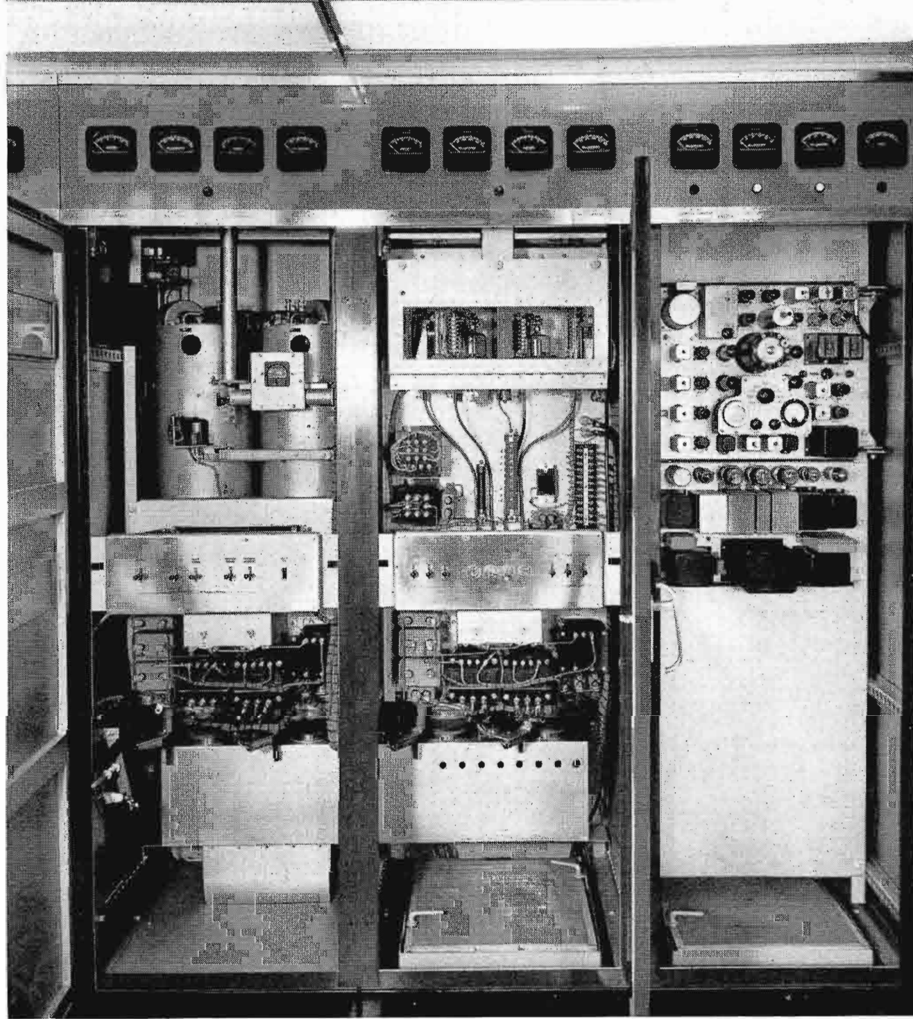
FIG. 6 (above). Closeup view of the "Direct FM" exciter at right, 1 and 3 KW low-power, grounded-grid amplifiers at center and 10 KW grounded-grid amplifier at extreme left.
