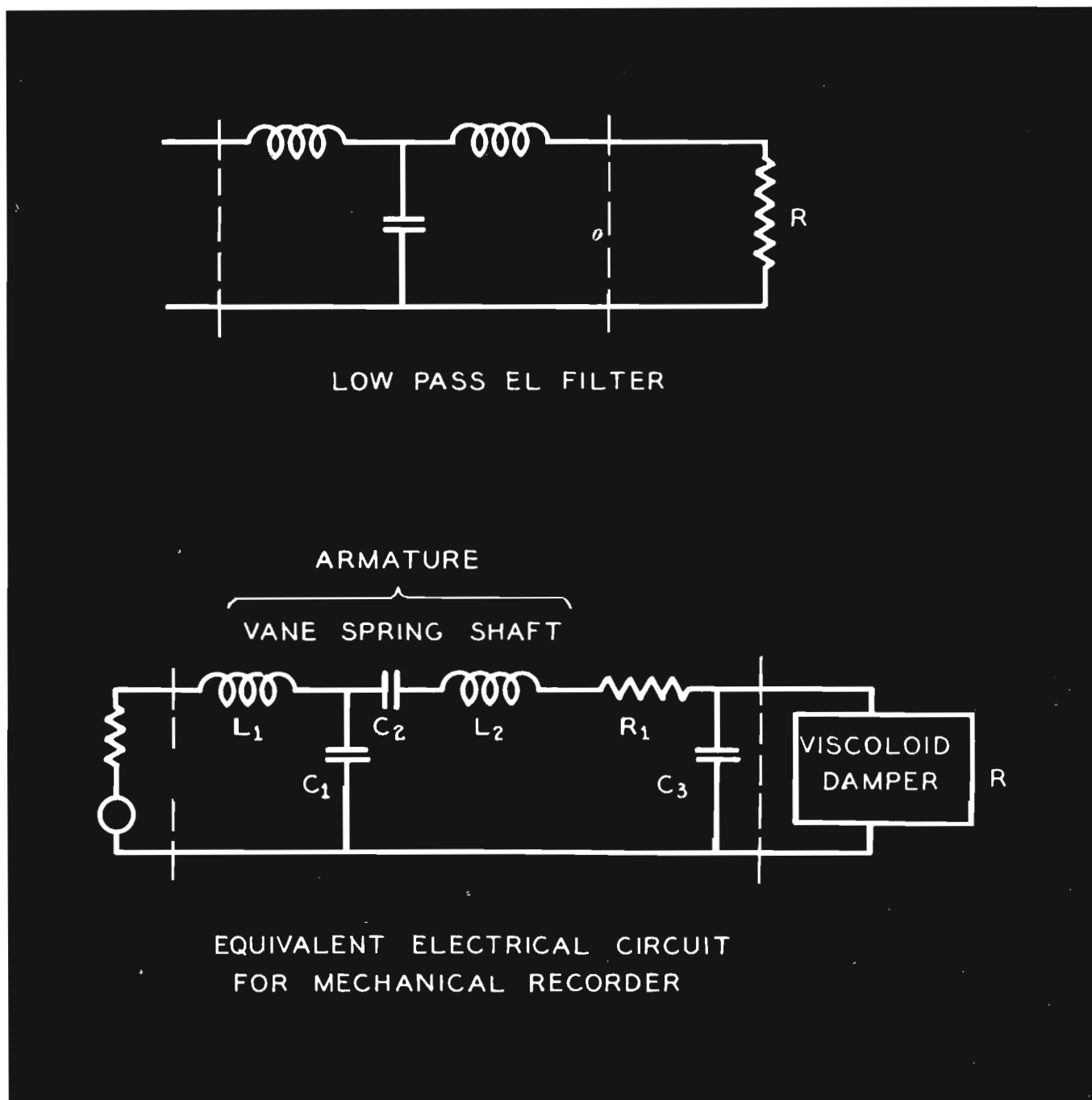
FIG. 2a. (Above) Low-Pass Electrical Filter.
